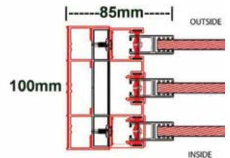
Single Glazing 8mm
