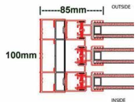
Double Glazing 20mm
