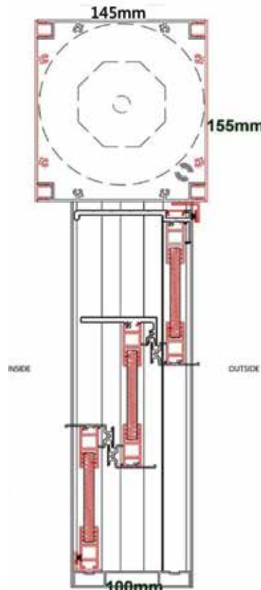
Double Glazing 20mm
